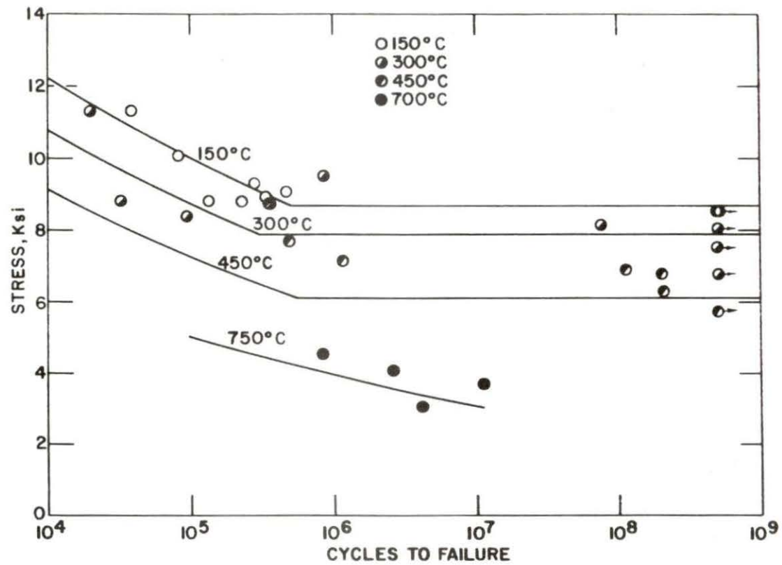
Fig. 6. S - N curves of swaged and annealed iodide zirconium
